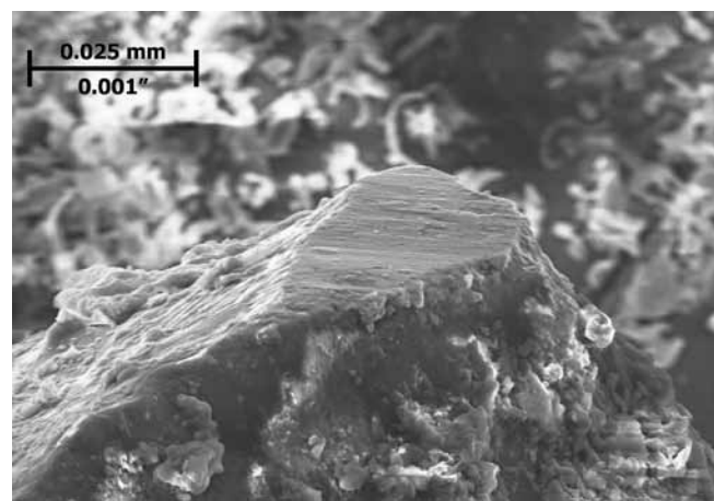
Figure 4: A dull grit in a worn, 46-mesh, vitrified-bond, N-grade, \text{Al}_2\text{O}_3 grinding wheel. Wheel dulling causes increased heat generation and grinding burn, increased normal forces and chatter and a finer surface finish.
