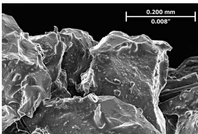
Figure 2: Sharp grits in a freshly dressed, 80-mesh, vitrified-bond aluminum-oxide grinding wheel. An 80-mesh, 16"-dia., 2"-wide, 2"-bore wheel contains about one billion abrasive grits.
