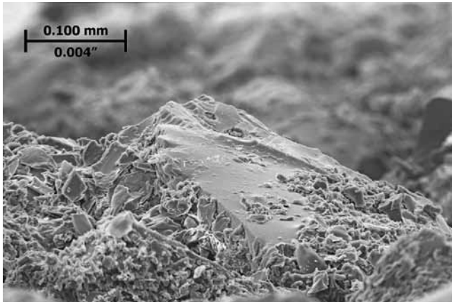
Figure 6: The tip of a microfracturing ceramic grit in a worn, 46-mesh, vitrified-bond, \text{Al}_2\text{O}_3 Norton-SG wheel after grinding hardened steel. This grit has done a lot of work, but it is not dull. Because it is a microfracturing grit, the tip of the grit remained sharp, enabling it to cut material efficiently.
