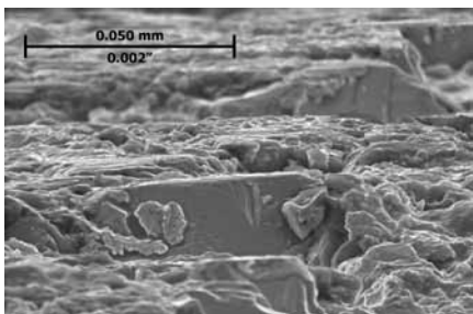
Figure 13: A worn, 140/170-mesh, resin-bond CBN wheel. Resin-bond wheels have little natural porosity. Here, only two grits can be seen poking above the bond material. "Sticking" the wheel clears some of the bond material, providing some porosity, but the wheel still has much less porosity than an electroplated or vitrified-bond wheel. As a result, cooling is more of a challenge and the wheels are more prone to mechanical loading.
