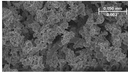
Figure 14: Swarf from using an \text{Al}_2\text{O}_3 wheel to continuous-dress grind a nickel-base alloy for making a turbine blade. Nickel-base alloys are very ductile, making the chips long and stringy.
