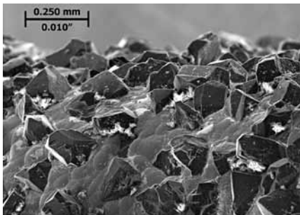
Figure 12: A worn electroplated CBN grinding wheel. Because electroplated wheels are not dressed, distribution of grit heights is random. This means that initially only the very highest grits are in contact with the workpiece, resulting in low grinding forces, low heat generation and a rough surface finish. As the wheel "closes down," the surface finish becomes finer and grinding power and heat generation both increase.
