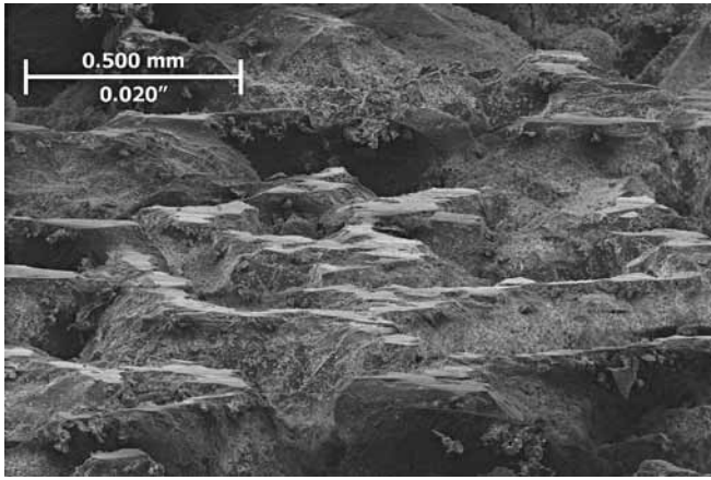
Figure 5: Dull grits in a worn, 46-mesh, vitrified-bond, N-grade, \text{Al}_2\text{O}_3 grinding wheel. This wheel was excessively dull, and the wear flats were visible to the naked eye. This N-grade wheel was "too hard," meaning it had too much bond material and dull grits did not break out of the bond.
