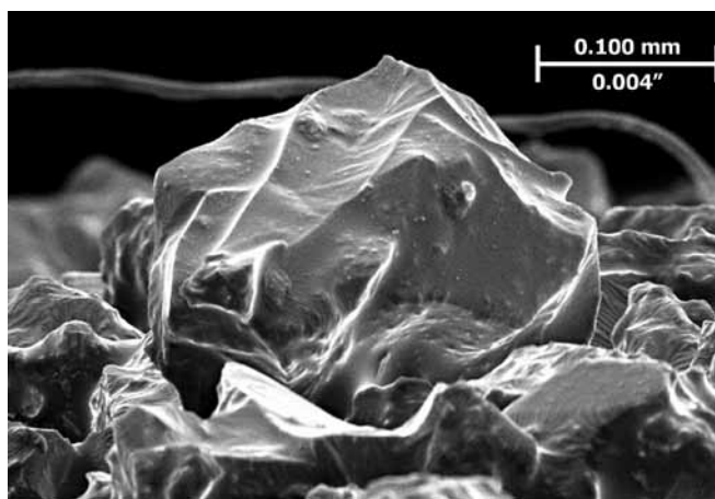
Figure 3: A single, 80-mesh \text{Al}_2\text{O}_3 grit in a freshly dressed vitrified-bond grinding wheel. A grit in a 16" wheel running at 3,000 rpm taking a 0.001" DOC is in contact with the workpiece 0.00008 seconds, or 0.08 milliseconds.
