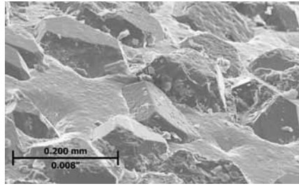
Figure 9: A worn electroplated diamond wheel for grinding tungsten-carbide dies. This wheel was at the end of its life, but not wheel dulling is visible. The wheel experienced a large amount of grit fracture and bond fracture, and the cutting-point density increased to such a degree that the grits no longer effectively penetrated the workpiece.
