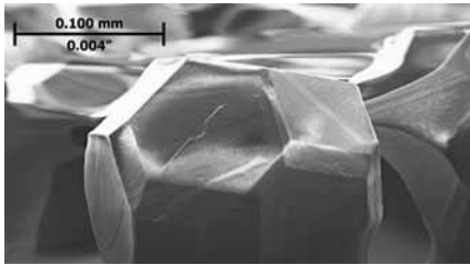
Figure 11: An 80/100-mesh diamond grit. Diamond and, in particular, cubic-boron-nitride abrasives can be manufactured in various geometries, from angular to blocky. This enables selection of geometries suited to particular grinding operations. The geometry shown is a truncated octahedron and is "blocky." Therefore, it is suitable for grinding operations requiring high material-removal rates.
