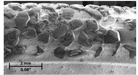
Figure 15: Diamonds in a worn rotary diamond disc. Some of the individual diamonds, about 1mm in diameter, have broken out of the binder material, which leads to dressing tool failure.
