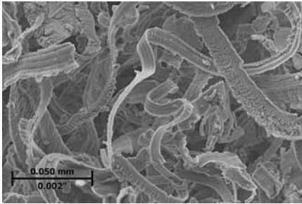
Figure 8: Swarf from grinding highly alloyed conventional HSS. Like turning and milling, grinding is a chip-formation process. However, the chips are thin and irregularly shaped. The swarf produced from grinding a standard ¼"-dia., 4"-long drill contains about 100 million individual chips.
