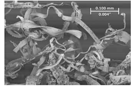
Figure 10: Swarf from grinding a tungsten-carbide workpiece with a resin-bond diamond wheel. Even grinding carbide, or "hard metal," is a chip-formation process. However, because of carbide's higher hardness and lower ductility compared to steel, the chips are shorter and blockier. Almost all grinding operations form chips. The exception is ceramic material, which has such low ductility that the material-removal mechanism isn't chip formation but rather brittle fracture. Ceramic material is removed when cracks form below the surface followed by the "beating out" of chunks of hard ceramic material above the cracks.
